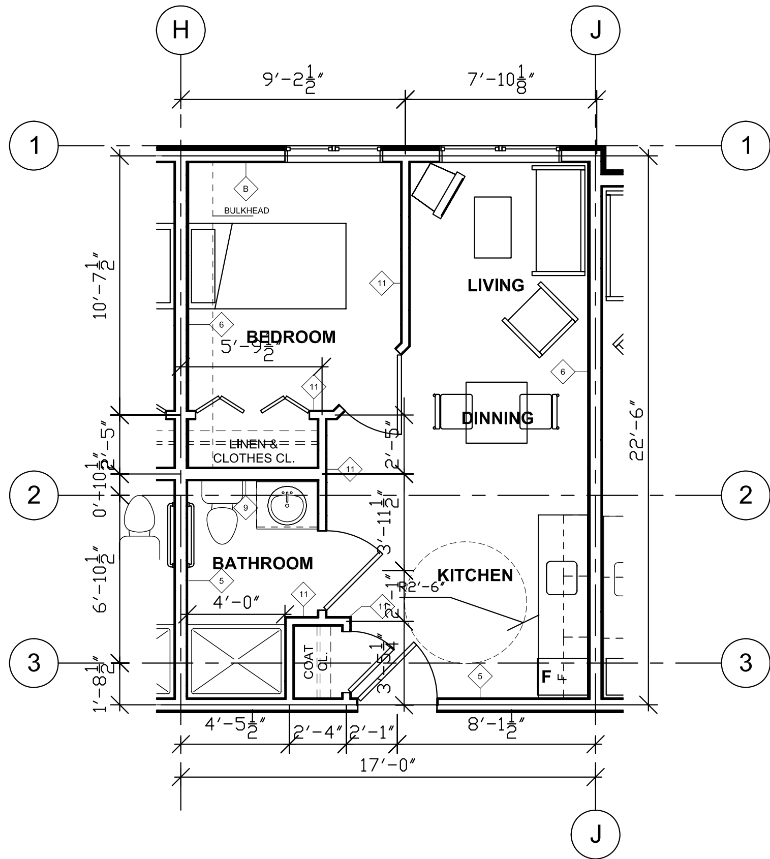
② UNIT Ab - 1 BEDROOM FLOOR PLAN 1/4" = 1'-0"
